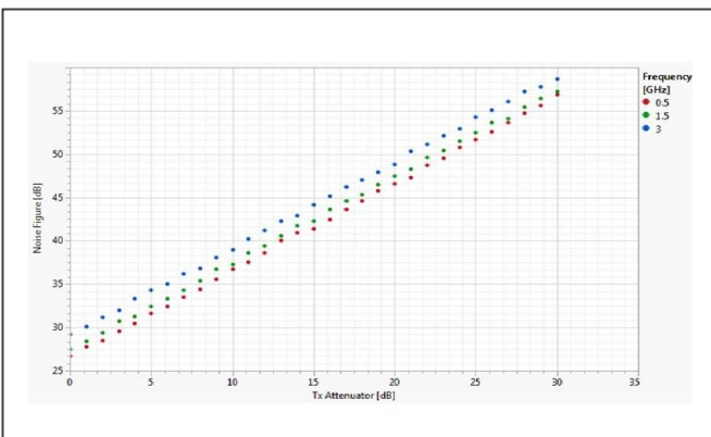
Noise Figure for 3 Freq. vs. Attenuator value, 3.0 GHz RFoF - 'LNA Off'
