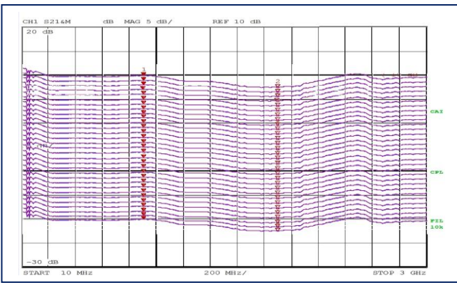
Gain vs. Tx Attenuation value: 0 to 31 dB in 1 dB step, 3.0 GHz RFoF for 'LNA Off' (similar behavior for 'LNA On')
