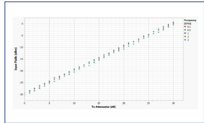
Input P1dBc at 5 frequencies, 3.0 GHz RFoF - 'LNA On'
