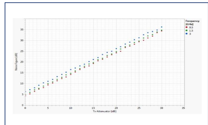
Noise Figure for 3 Freq. vs. Attenuator value, 3.0 GHz RFoF - 'LNA ON'
