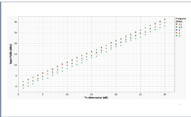
Input P1dBc at 5 frequencies, 3.0 GHz RFoF - 'LNA Off'
